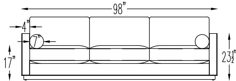
3 X 3 SEAT @ BACK
