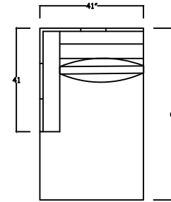
180807L ONE ARM CHAISE * PLINTH BASE flush on connected side * SHOWN AS LEFT
